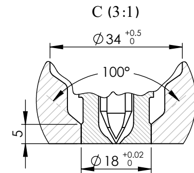
Detail view of nozzle's injection point
