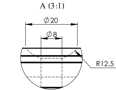
Detail view of nozzle's entry
