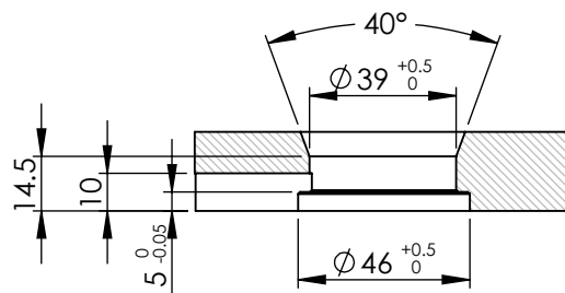
B : Detail view of injection ring
