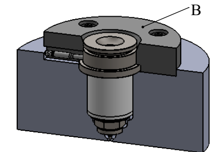
Isometric view of nozzle's placement in the mold
