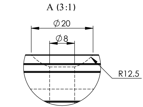
Detail view of nozzle's entry
