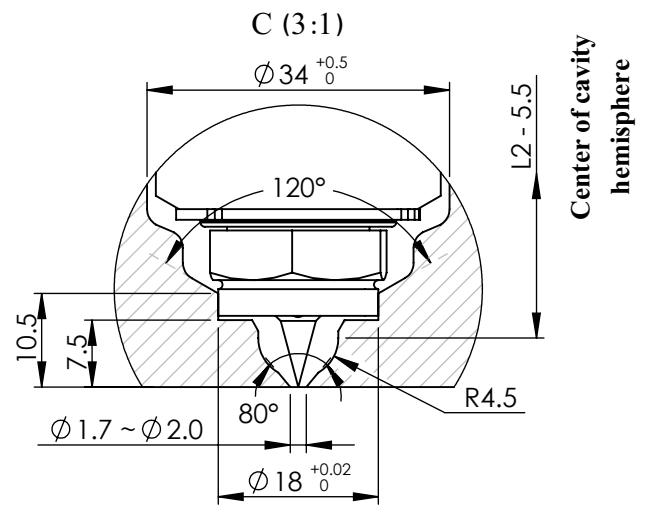
Detail view of nozzle's injection point
