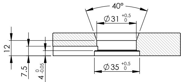
B : Detail view of injection ring
