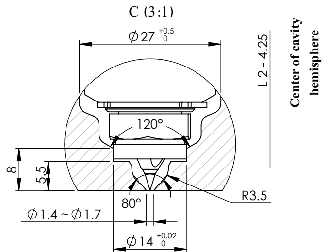
Detail view of nozzle's injection point
