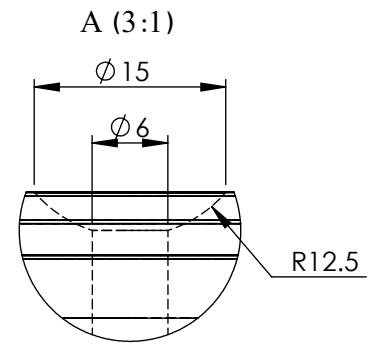
Detail view of nozzle's entry
