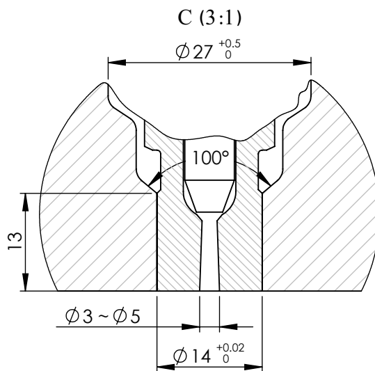
Detail view of nozzle's injection point
