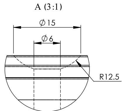
Detail view of nozzle's entry
