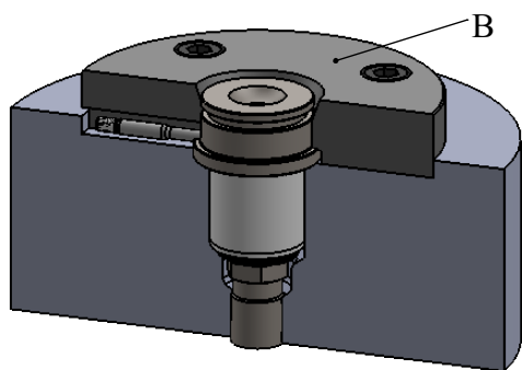
Isometric view of nozzle's placement in the mold
