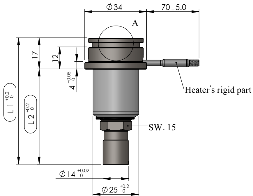
Detail view of nozzle's entry
