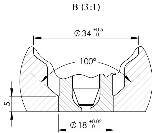
Detail view of nozzle's injection point
